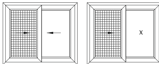
Sliding flyscreen
